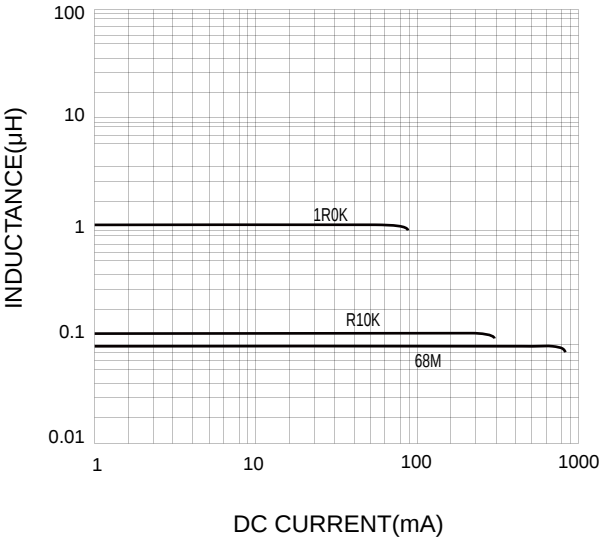
Inductance VS. DC Current Charcteristics:
