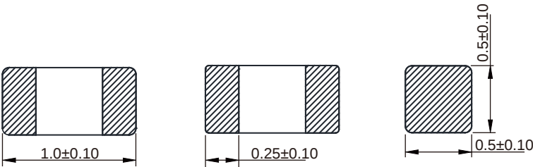
Dimensions: [mm]
