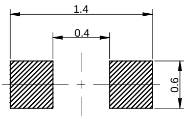
Land Pattern: [mm]
